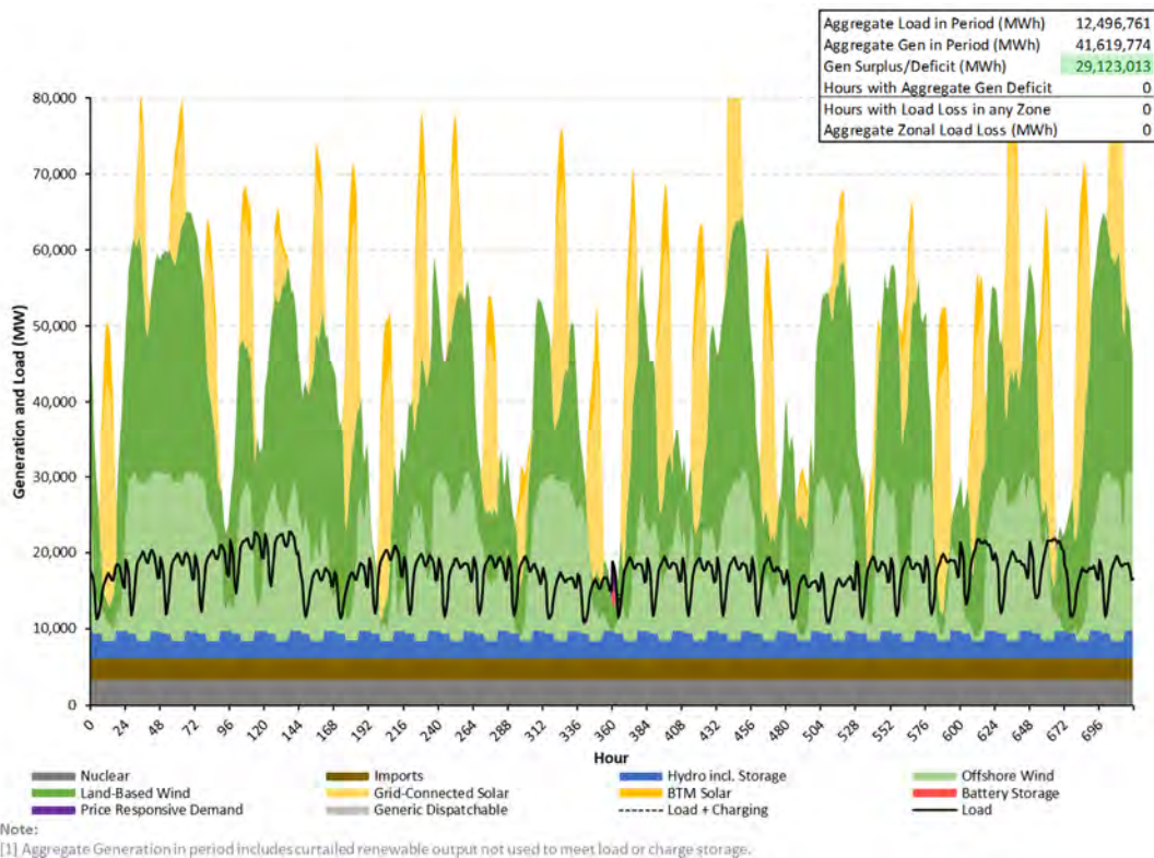
Figure 34: Hourly Load/Generation Balance, CCP2-CLCPA Shoulder
