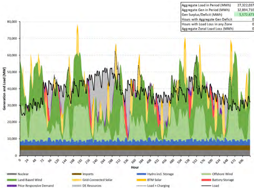
Figure 30: Hourly Load/Generation Balance, CCP2-CLCPA Winter
